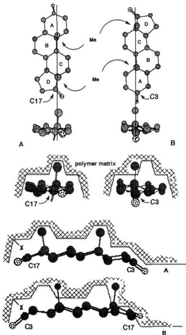
Figure 1. (Top) Match (A) and mismatch (B) of 1 in a cavity which originates from 4c . (Bottom) Side view of 1 showing match (A) and mismatch (B) in a cavity (from 4c ). The reagent X reacts from the desired side of the substrate molecule 1 when this fits properly into the cavity.
